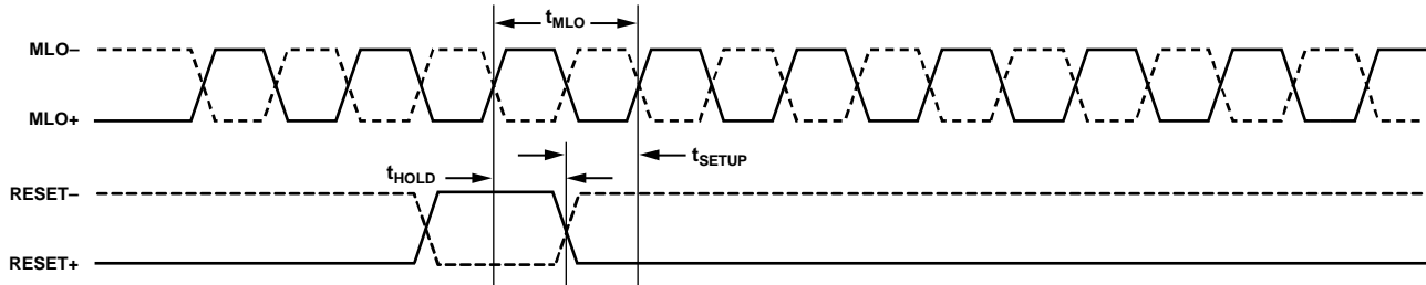
Figure 6. CW Doppler Mode Input MLO±, Pulse Asynchronous RESET± Timing, 4LO/8LO/16LO Mode
