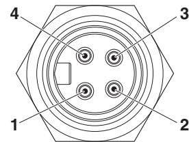
Pin assignment, plug, 7/8"-16UNF, 4-pos., view of male side
