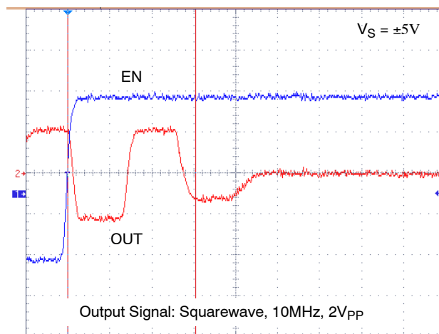
Figure 25. Turn OFF Time Delay Vertical: (EN) 500mV/div (OUT) 1V/div Horizontal: 40ns/div
