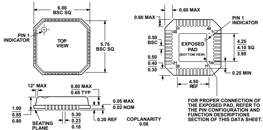
Figure 135. 40-Lead Lead Frame Chip Scale Package [LFCSP_VQ]
