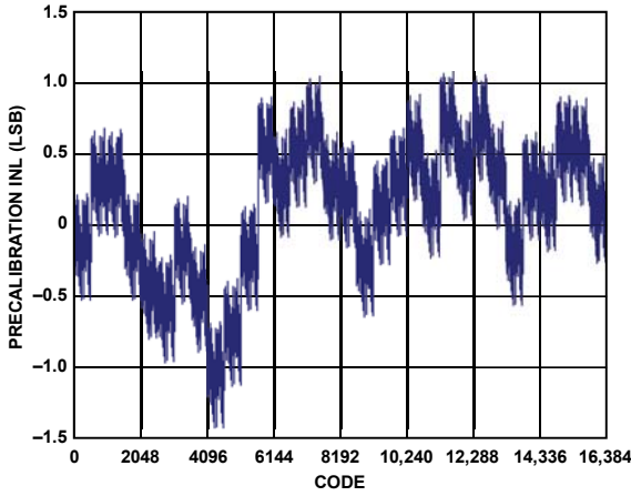
Figure 6. AD9717 Precalibration INL at 1.8 V (DVDD = 1.8 V)
