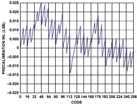
Figure 30. AD9714 Precalibration INL at 1.8 V
