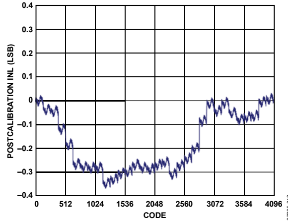
Figure 21. AD9716 Postcalibration INL at 3.3 V
