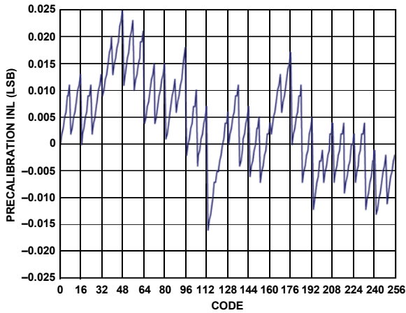
Figure 32. AD9714 Precalibration INL at 3.3 V
