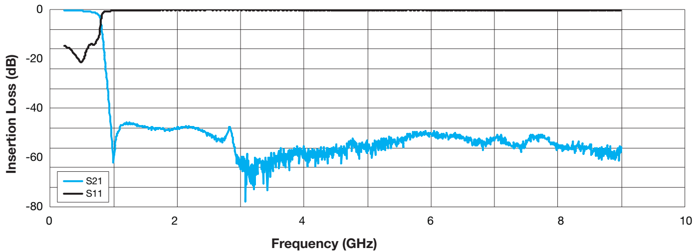
Typical Frequency Response
