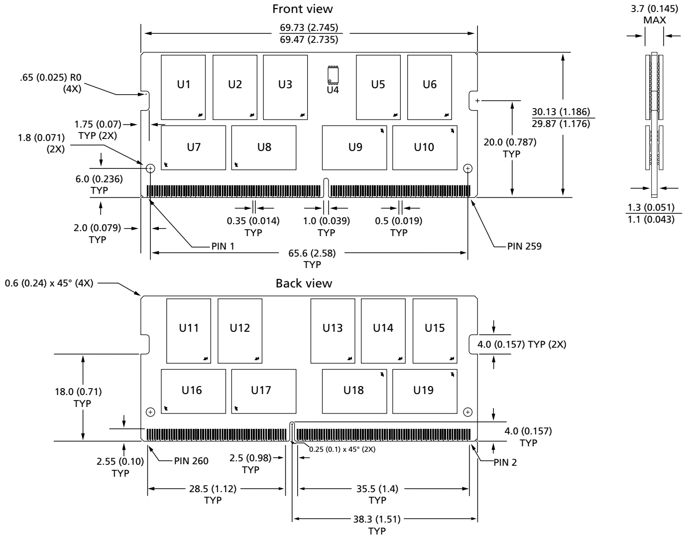
Figure 6: 260-Pin DDR4 SODIMM (R/C-H)
