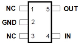
SC-88A (SC-70-5) (Top View)
